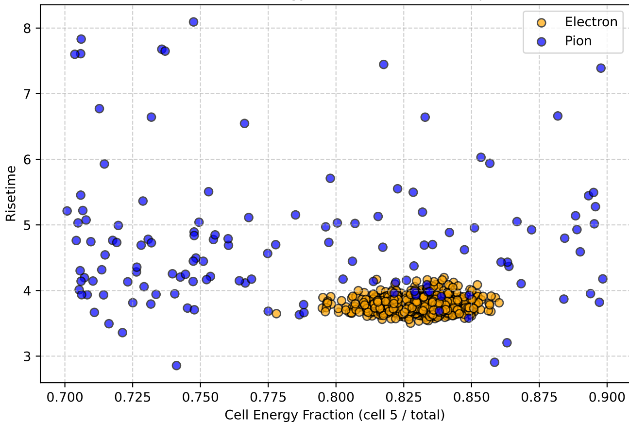
Risetime vs Cell Energy Fraction for 40.0GeV particles
